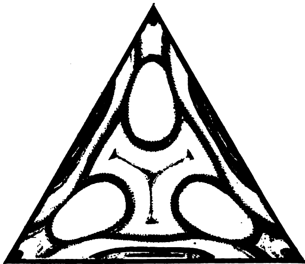
ISOCROMATIC LINES IN A TRIANGLE OF UNANNEALED GLASS.
